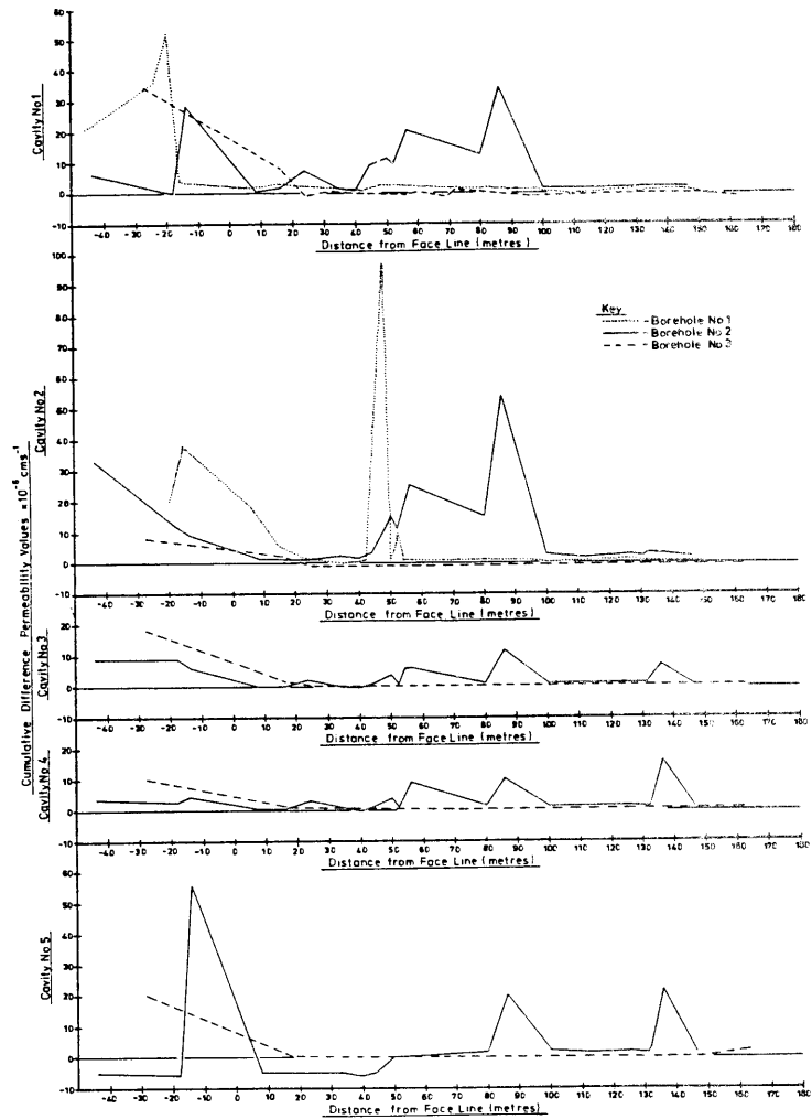
Figure 9 Cumulative Difference Permeability Values for the Bagworth Test Cavities against Distance from Face Line
